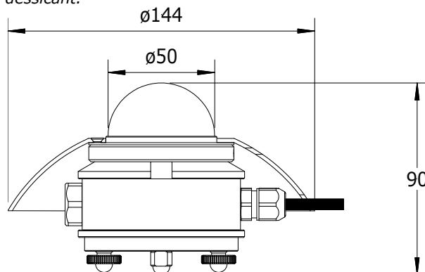
Figure 1 SR11 solar radiation sensor. (1) sensor, (2, 3) glass domes, (5) cable, standard length 5 m, (9) desiccant.
