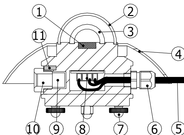
Figure 1 SR11 solar radiation sensor. (1) sensor, (2, 3) glass domes, (5) cable, standard length 5 m, (9) desiccant.
